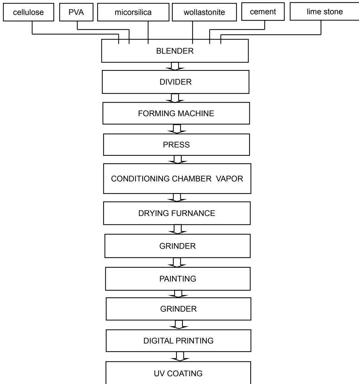
Fig. 2. A scheme of manufacturing of the SCALAMID decorative finishing panels by POZ BRUK Sp. z o.o. Sp.j. in factory in Sobota (Poland).
