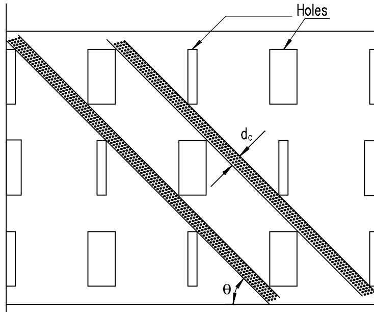
Figure 3: Depth d_c of a continuous strut
