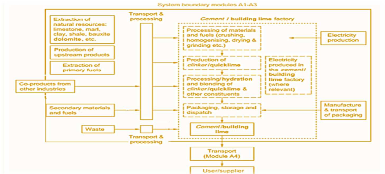
Figure 1. Inputs and processes of product system.
