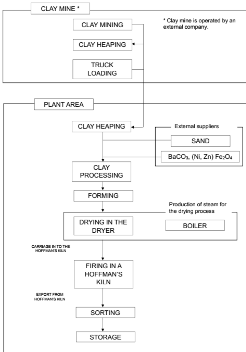
Fig. 1. The scheme of the ceramic tiles production process by Patoka.
