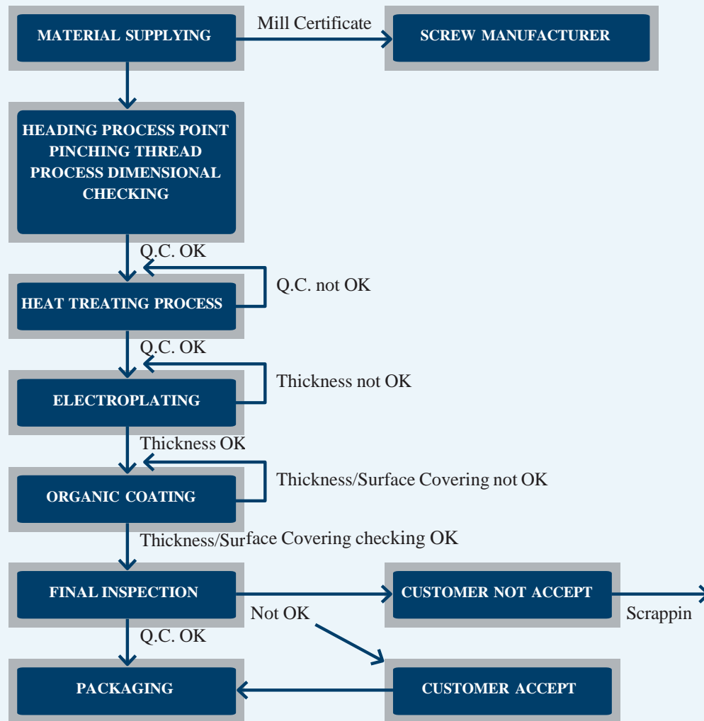
Figure 3.Screws- Manufacturing process
