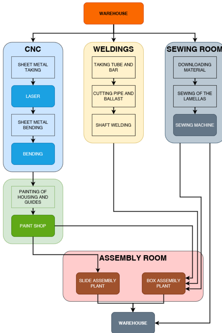
Figure 3 Manufacturing process scheme (A3)
