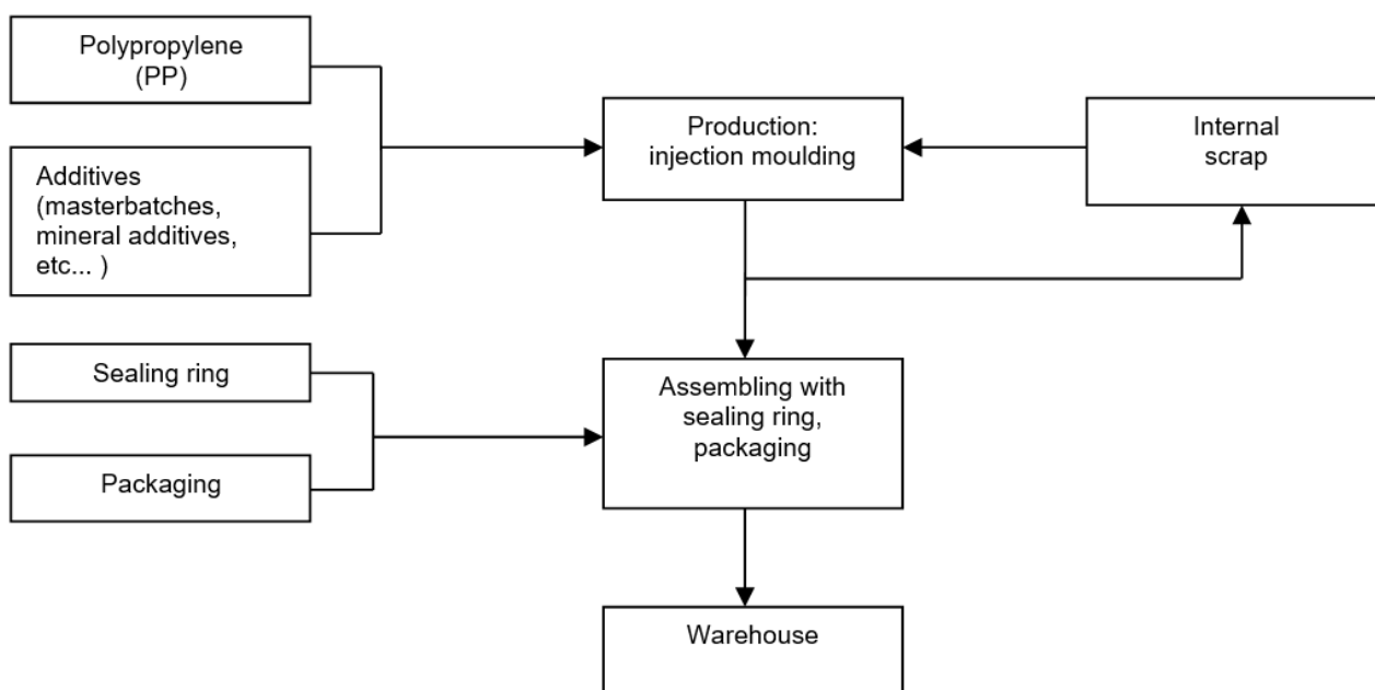
Figure 3. Diagram of the manufacturing process of production site Kartoszyño.
