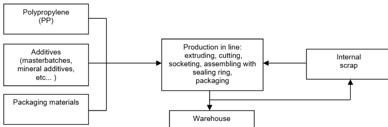
Figure 2. Diagram of the manufacturing process of production site Strzałków.
