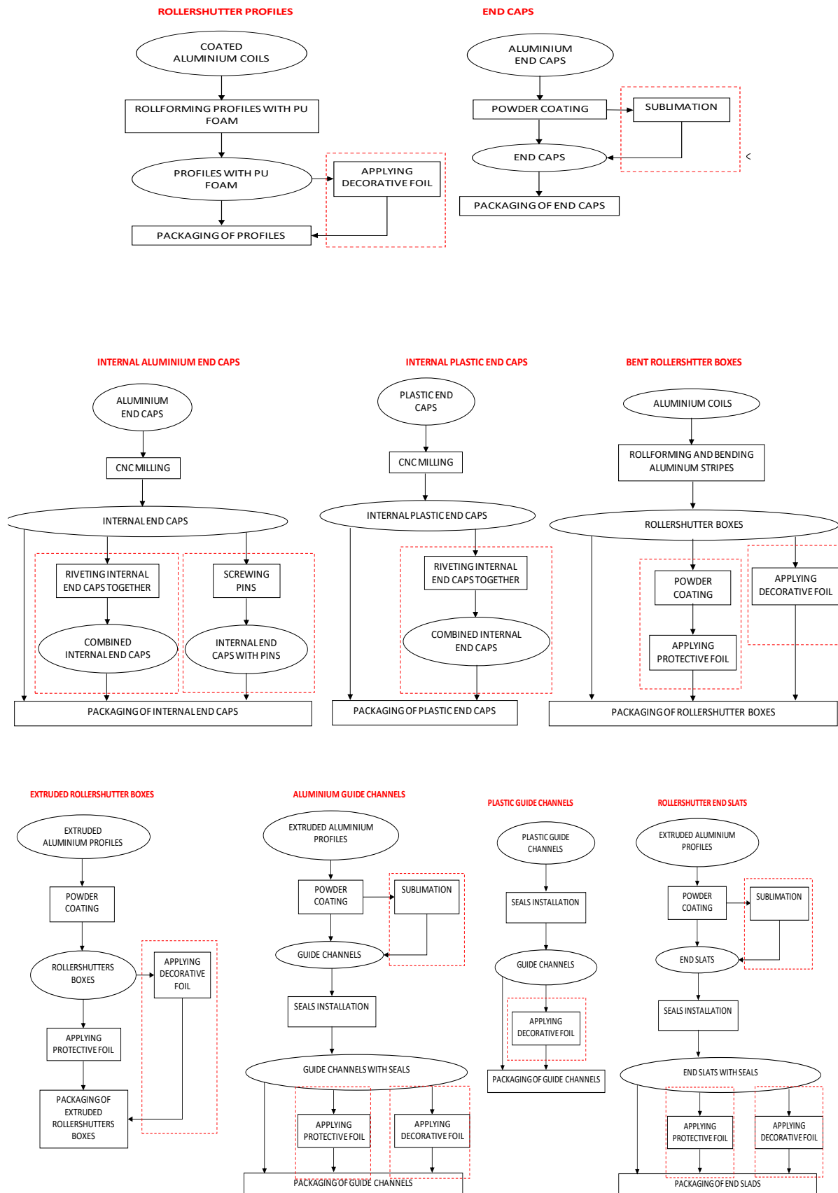
Figure 2. A schematic diagram of the industrial process in Opole (A3)
