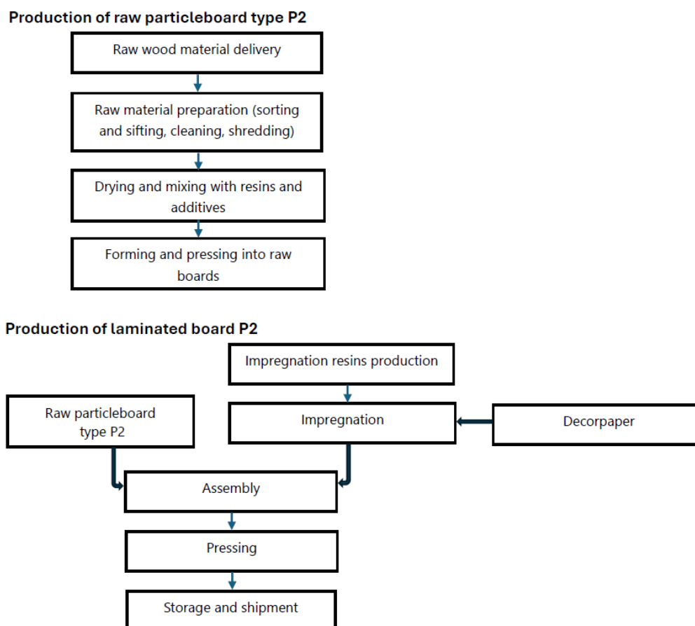
Fig. 3. A scheme of laminated - board P2 process production by Woodeco (Poland).
