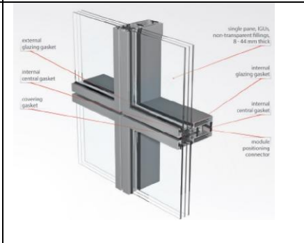
PROCURAL PF173 MODULAR FAÇADE
