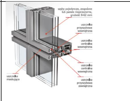
MODULAR FAÇADE PROCURAL PF173N
