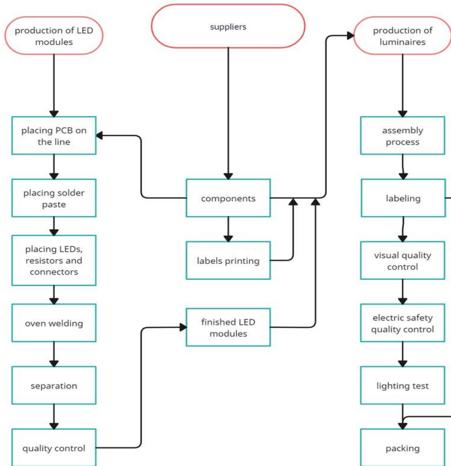
Fig. 3. A basic scheme of the LED luminaire/plastic product manufacturing process
