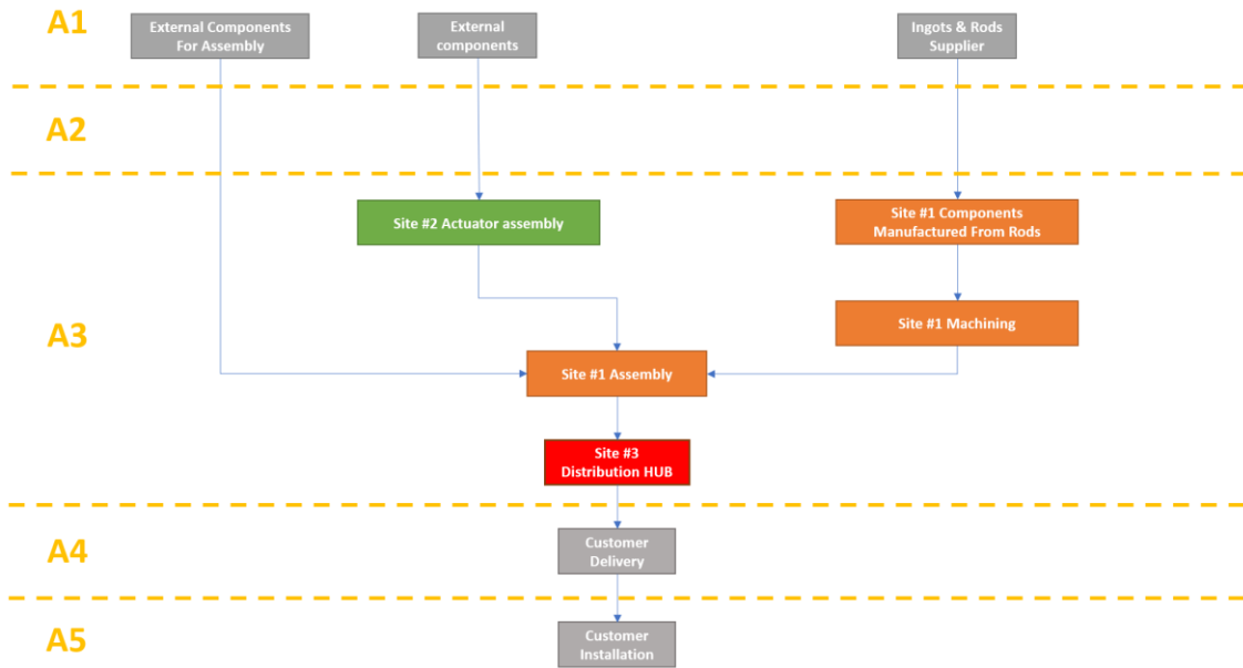
Figure 2 Manufacturing process scheme (A1-A3), with forming/assembly process in Ljung (Sweden) (A3)
