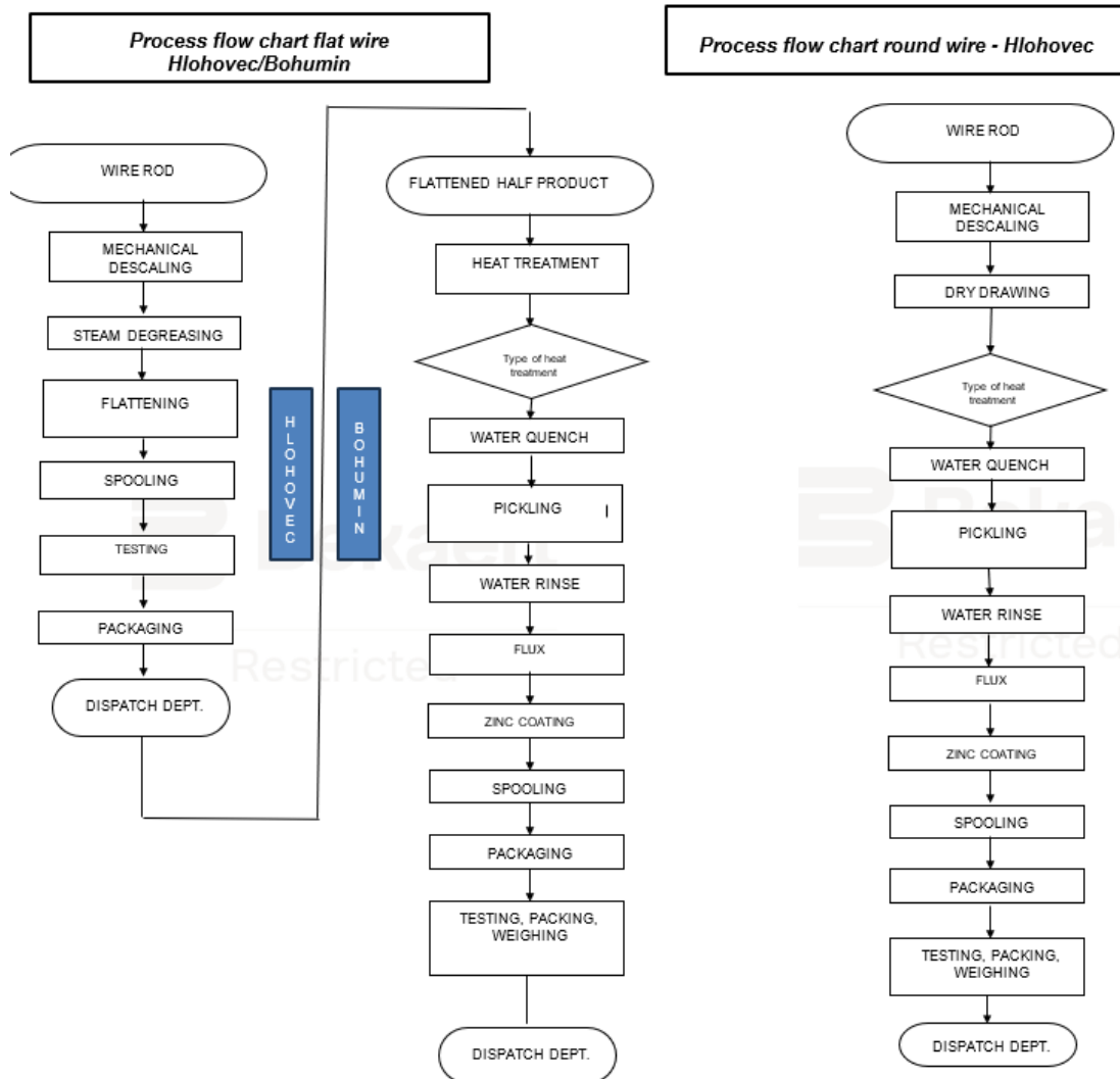
Fig. 1. Production process for flat and round products
